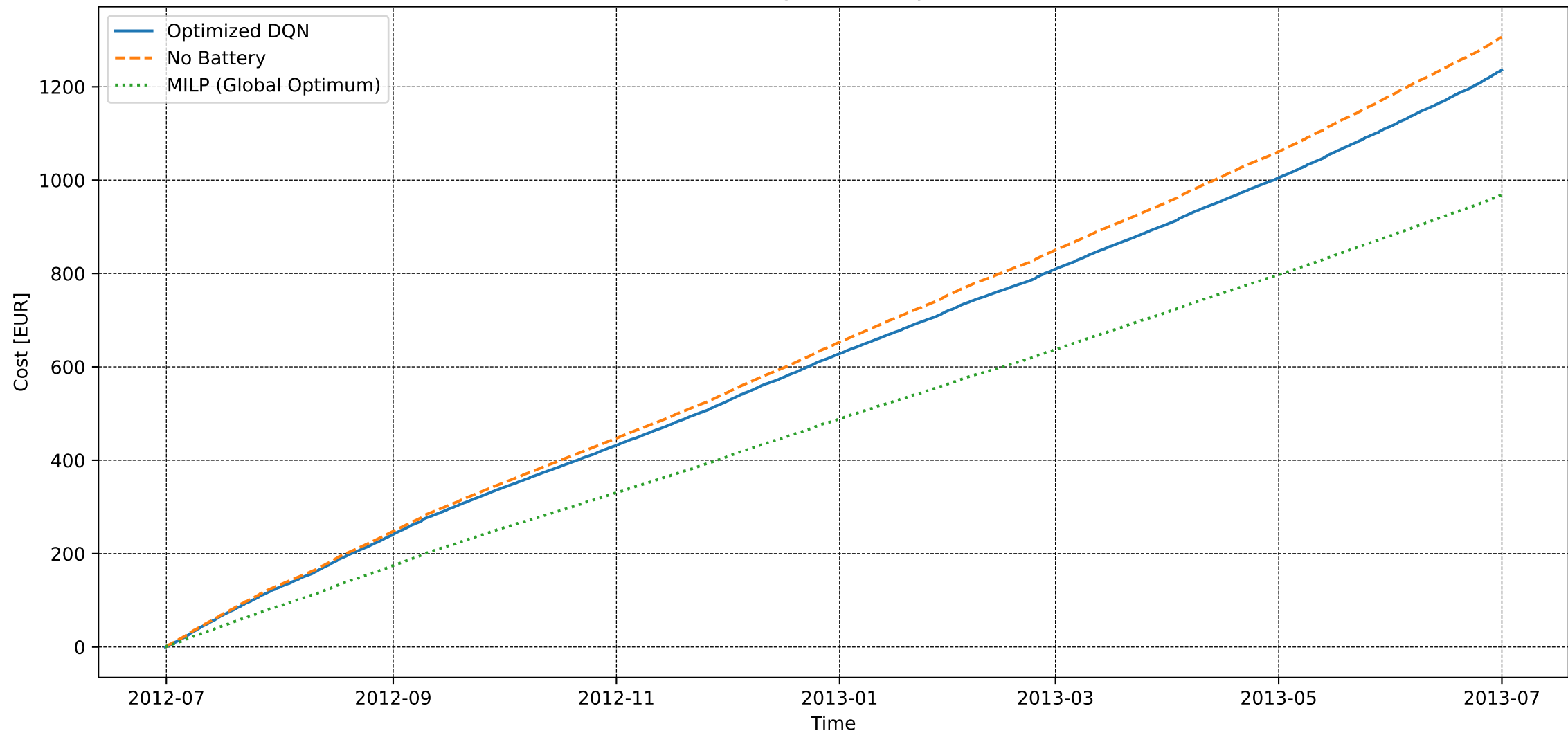
User 128 - Basic Training - Electricity Cost [DQN vs MILP]
